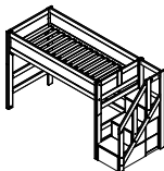
LOW-LOFT BED WITH STEPLADDER H 152 x W 257 x D 102 Ground clearance below the bed 113 CM
